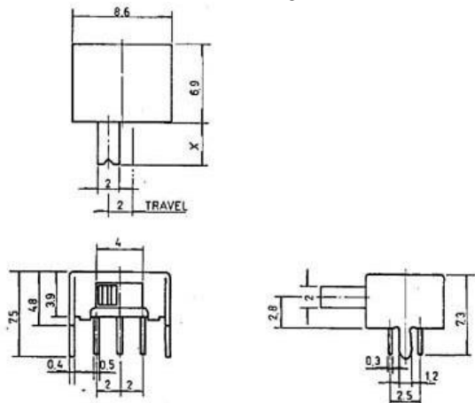
Outline Drawing
