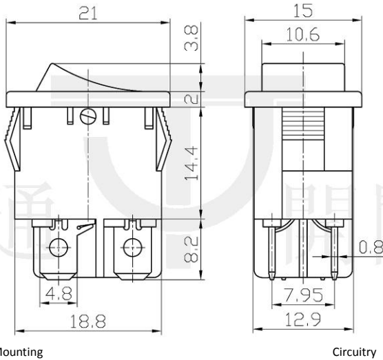
Outline Drawing
