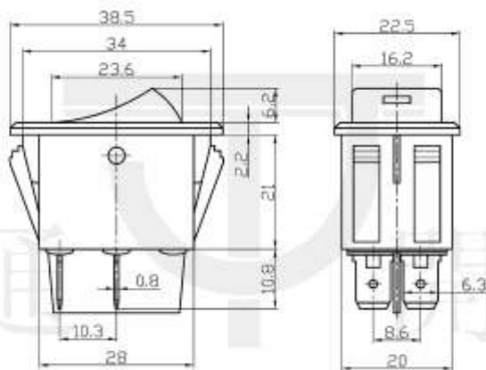
Outline Drawing
