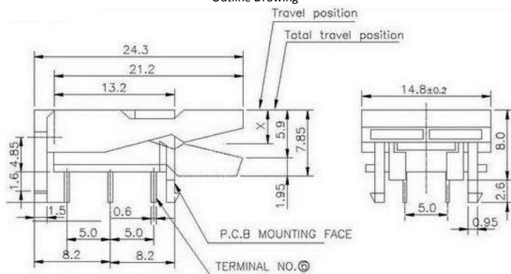
Mounting
