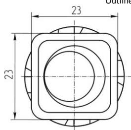
Outline Drawing
