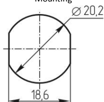
Mounting
