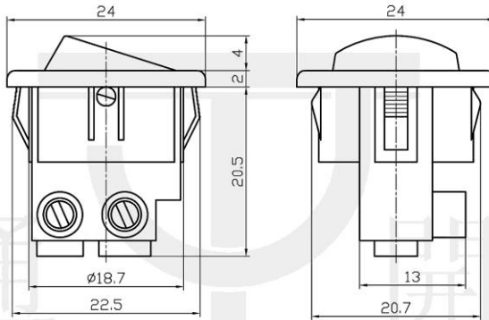
Mounting
