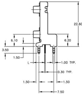
Outline Drawing
