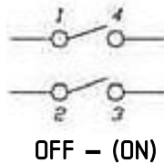
L=3,85mm Circuitry
