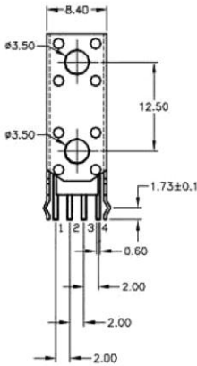
Mounting
