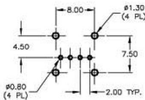
Mounting
