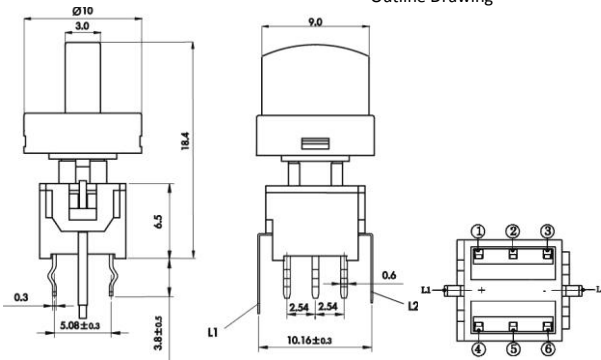
Outline Drawing
