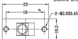
Outline Drawing
