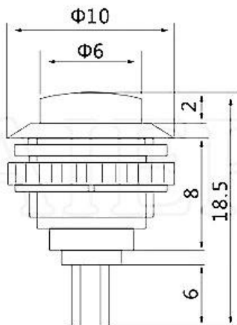
Outline Drawing
